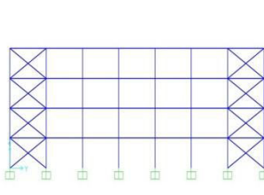
Fig 3.8 YZ Plane
