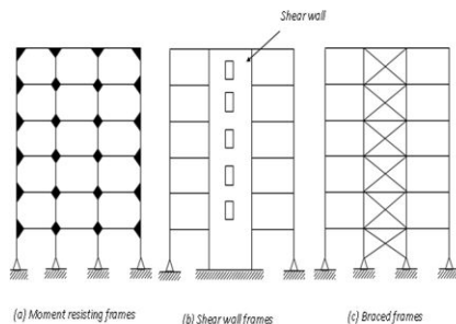
Fig 3.3 Lateral load resisting system
