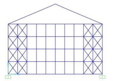
Fig 3.7 XZ Plane
