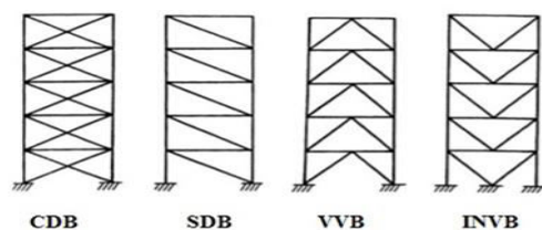
Fig 3.6 Bracing systems
