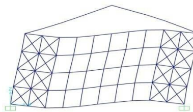
Fig 3.9 Deformed shape of 1 st mode (t=0.834)
