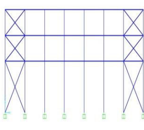
Fig 4.1 CDB in YZ plane
