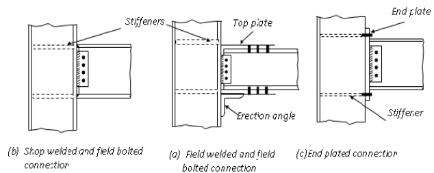
Fig. 3.3.1) Moment resistant connections
