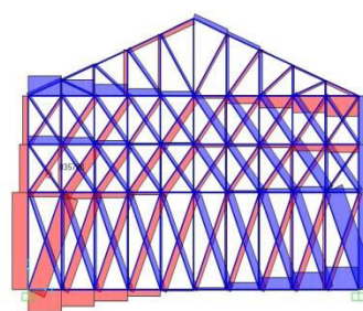
Fig 4.2 AFD in Howe type of truss
