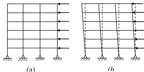
Fig 3.2 Multi-storey frame without lateral bracing
