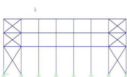
Fig 4.6 VVB Deformed shape 1 st mode (t=0.581)
