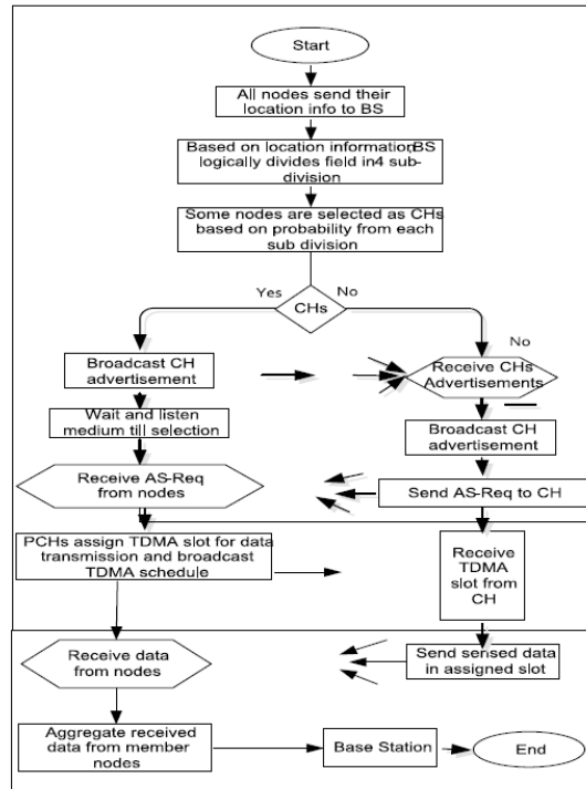
Fig. 1. Working Principle of Q-LEACH
