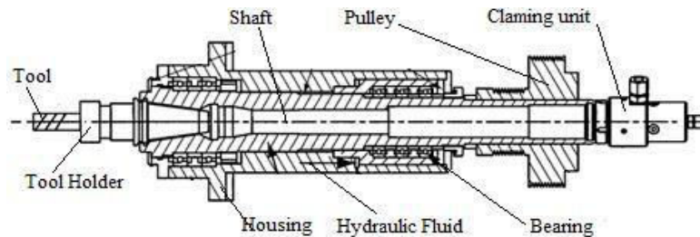
Figure 1: Elements in a Spindle System
