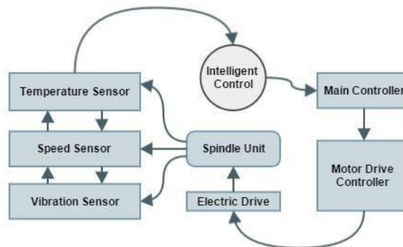
Figure 2: Vibration Control in Spindle System
