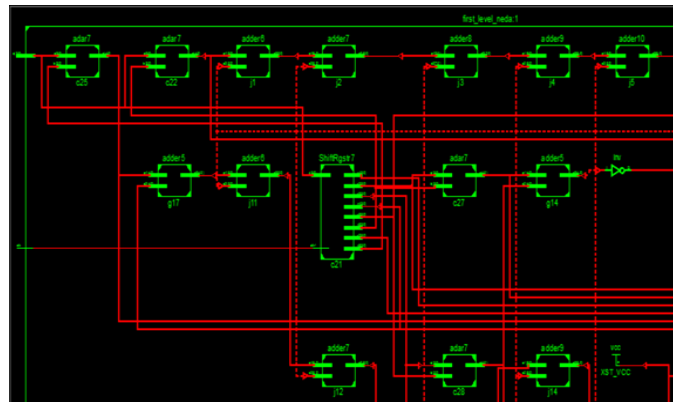
Figure 4: RTL View of 1-D Wavelet Transform
